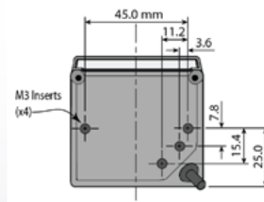
HOLE TOLERANCE: +/- 0.1 MM BOTTOM VIEW
